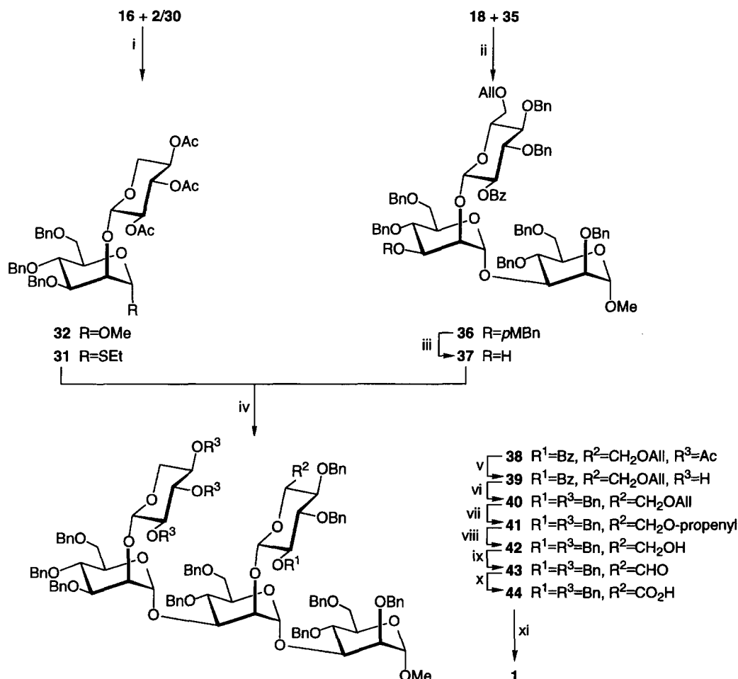
Scheme 2. Reagents and conditions: (i) TMSOTf, 1,2-dichloroethane, -40^{\circ}\text{C}\rightarrow 20^{\circ}\text{C} , 31 5 h, 38%, 32 1 h, 68%; (ii) NIS/TfOH (cat.), 1,2-dichloroethane-Et 2 O, -30^{\circ}\text{C} , 15 min, 81%; (iii) DDQ, dichloromethane-water, 1 h, 82%; (iv) see ii, 0^{\circ}\text{C} , 67%; (v) KO t -Bu, MeOH, 20 h, 73%; (vi) BnBr, NaH, DMF, 3 h, 88%; (vii) Ir(COD)[PCH 2 (Ph) 2 ] 2 PF 6 , 1,2-dichloroethane, 70 h; (viii) HCl-MeOH (0.5 M), 22 h, 78% (over 2 steps); (ix) ClCOCOCl, DMSO, 1.5 h; (x) NaClO 2 , 2-Me-2-butene, NaH 2 PO 4 , t -BuOH, water, 20 h; (xi) Pd(C), H 2 , t -BuOH-water, 38 h, 57% (over 3 steps).
