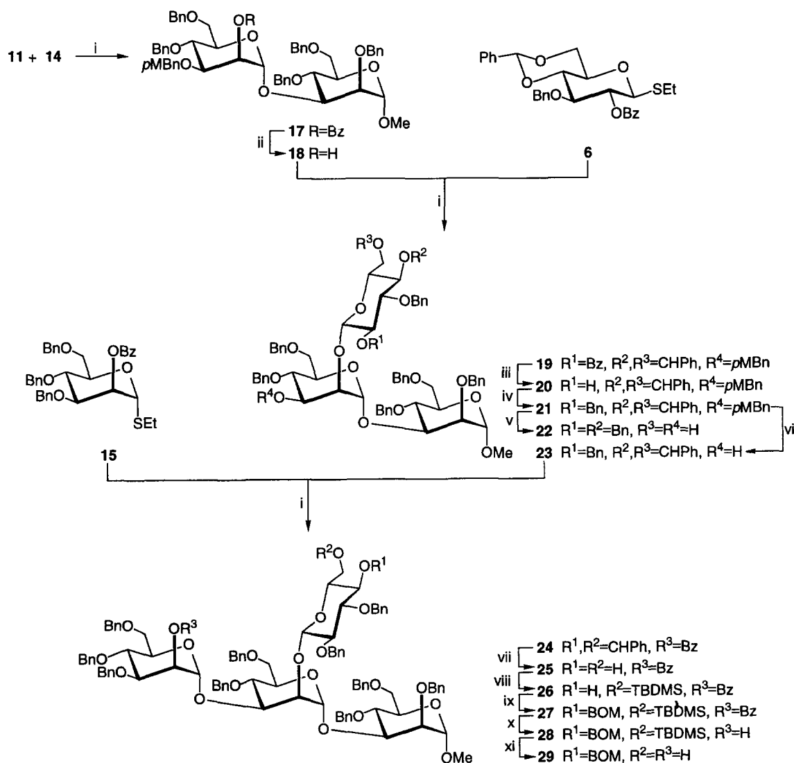
Scheme 3. Reagents and conditions: (i) NIS/TfOH(cat.), 1,2-dichloroethane-Et 2 O, 0 °C, 15 min, 17 84%, 19 88%, 24 94%; (ii) KOt-Bu, MeOH, 48 h, 85%; (iii) KOt-Bu, MeOH, 96 h, 98%; (iv) BnBr, NaH, DMF, 85%; (v) AlCl 3 , Et 3 N·BH 3 , toluene, 30 min, 42%; (vi) DDQ, dichloromethane–water, 3 h, 75%; (vii) 80% HOAc, reflux, 2 h, 83%; (viii) TBDMSCl, DMAP, pyridine, 20 h, 78%; (ix) BOMCl, DIPEA, n -Bu 4 Nl, CH 3 CN, 18 h, 76%; (x) KOt-Bu, dioxane–MeOH, 55 h, 92%; (xi) TMSOTf, 1,2-dichloroethane, –40 °C→20 °C, 5.5 h, 73%.
