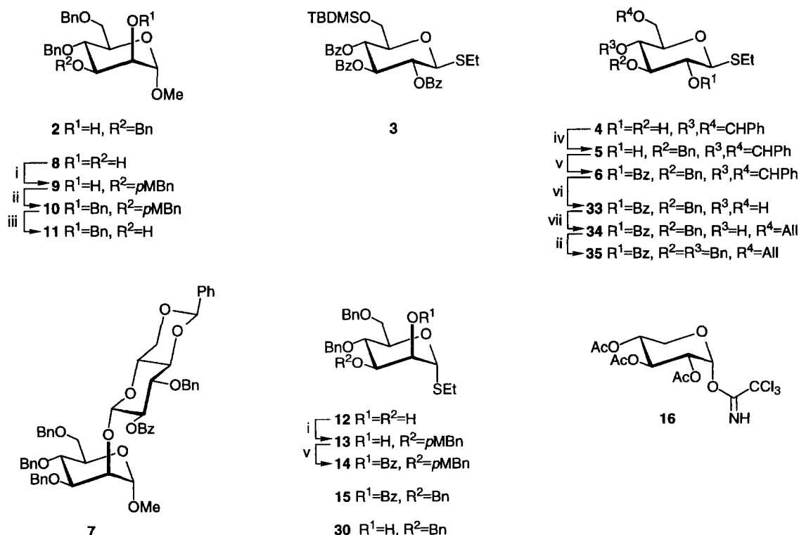
Scheme 1. Reagents and conditions: (i) Bu_3SnO , MeOH, reflux, 1.5 h; pMBnCl , CsF, NaI, DMF, 17 h, 9 79%, 13 75%; (ii) BnBr , NaH, DMF, 17 h, 10 97%, 35 82%; (iii) DDQ, dichloromethane–water, 1 h, 81%; (iv) Bu_3SnO , MeOH, reflux, 1.5 h; BnBr , CsF, DMF, 17 h, 84%; (v) BzCl , pyridine, 1.5 h, 6 88%, 14 87%; (vi) 80% HOAc, 1 h, 85%; (vii) Bu_3SnO , MeOH, reflux, 1.5 h; AllBr , CsF, DMF, 18 h, 78%.
